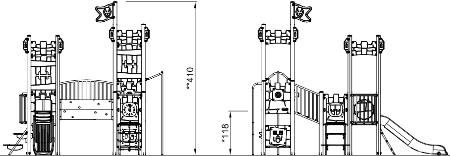
PCM400700 1:100
